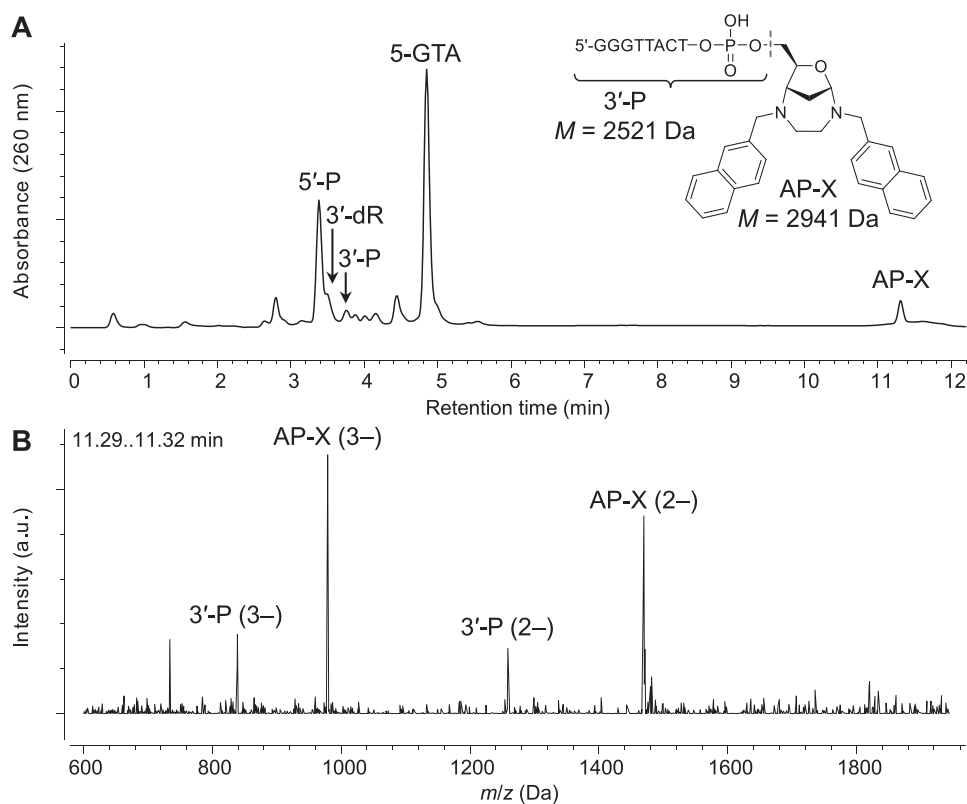
Figure 4. (A) UV-UPLC analysis of products obtained upon reaction of AP duplex (20 \mu\text{M} ) with C2N2 (40 \mu\text{M} ) in 15 mM \text{KAsO}_2\text{Me}_2 , 115 mM KCl, pH 6.5 buffer. Whenever possible, the peaks were assigned on the basis of their mass spectra. (B) Mass spectrum ( \text{ESI}^- ) of the UPLC peak with t_R = 11.30 min (AP-X). The peaks attributed to 3'-P presumably arise from fragmentation of AP-X, shown by the dashed line in panel (A).
