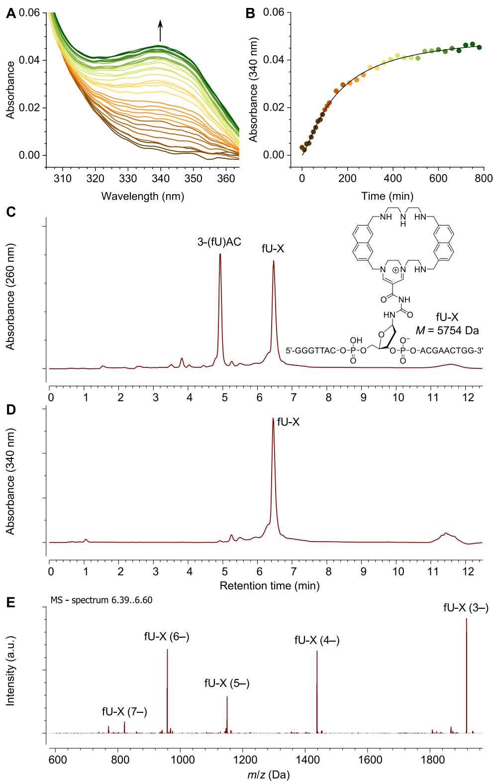
Figure 6. (A–B) Changes of in absorption spectra (A) and time course (B) of the reaction of fU duplex (3-(fU)AC/5-GTA, 10 \mu M) with BisNP-NH (20 \mu M) in 15 mM \text{KAsO}_2\text{Me}_2 , 115 mM KCl buffer, pH 7.2, reaction temperature: 37°C. (C–D) UV-UPLC analysis of reaction of the fU-containing strand 3-(fU)AC (20 \mu M) with BisNP-NH (40 \mu M) performed in the conditions described above, detected at the wavelengths of 260 nm (C) and 340 nm (D). (E) Mass spectrum (ESI - ) of the UPLC peak with t_R = 6.50 min (fU-X). The putative structure of the fU-X adduct is shown as inset in (C).
