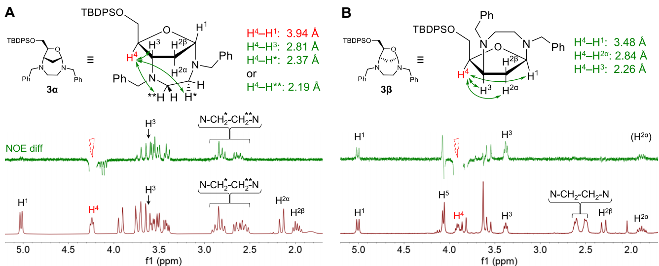
Figure 3. Structures of 3 \alpha (A) and 3 \beta (B) indicating selected interatomic distances (according to molecular models, cf. Supplementary Figure S16) and observed NOE couplings (green arrows). In 3 \alpha , two clusters of conformations were observed differing by the pucker of the ethylenediamine bridge and the proximity of either H^* or H^{**} to H^4 (cf. Supplementary Note 1). Bottom panels: ^1H NMR (300 MHz, CDCl_3 , dark red) and 1D NOE difference spectra (green) obtained by selective irradiation of H^4 protons.
