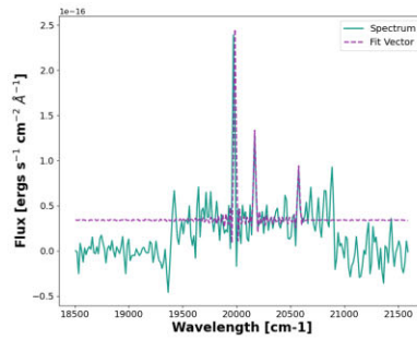
(e) SN2 spectrum and fitted vector for incorrectly categorized PNe region
