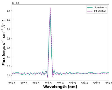
(d) SN1 spectrum and fitted vector for incorrectly categorized SNR region
