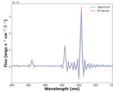
(b) SN2 spectrum and fitted vector for correctly categorized PNe region
