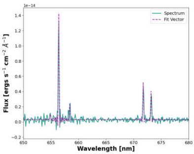
(c) SN3 spectrum and fitted vector for correctly categorized SNR region
