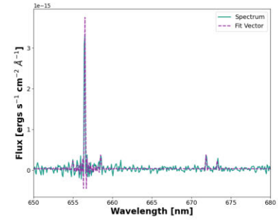
(c) SN3 spectrum and fitted vector for correctly categorized PNe region
