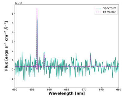
(f) SN3 spectrum and fitted vector for incorrectly categorized PNe region
