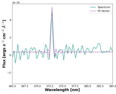
(a) SN1 spectrum and fitted vector for correctly categorized PNe region
