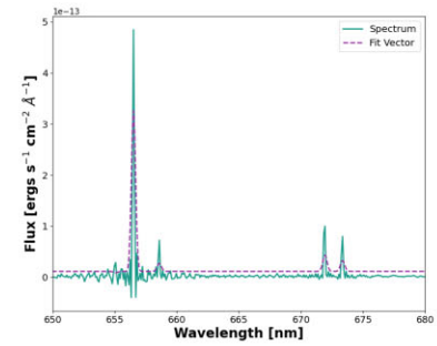
(f) SN3 spectrum and fitted vector for incorrectly categorized SNR region
