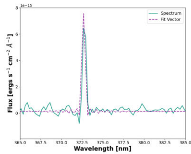
(a) SN1 spectrum and fitted vector for correctly categorized SNR region
