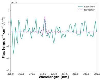
(d) SN1 spectrum and fitted vector for incorrectly categorized PNe region
