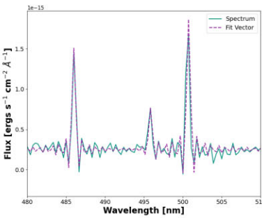
(b) SN2 spectrum and fitted vector for correctly categorized SNR region
