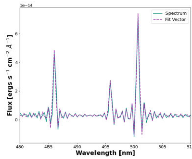
(e) SN2 spectrum and fitted vector for incorrectly categorized SNR region
