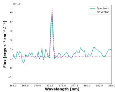
(d) SN1 spectrum and fitted vector for incorrectly categorized H II region
