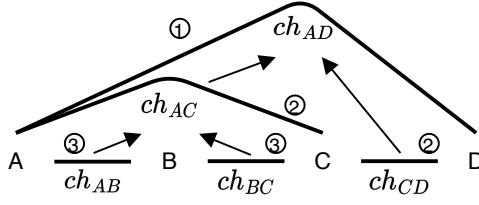
Fig. 11. Recursive construction of virtual payment channels
