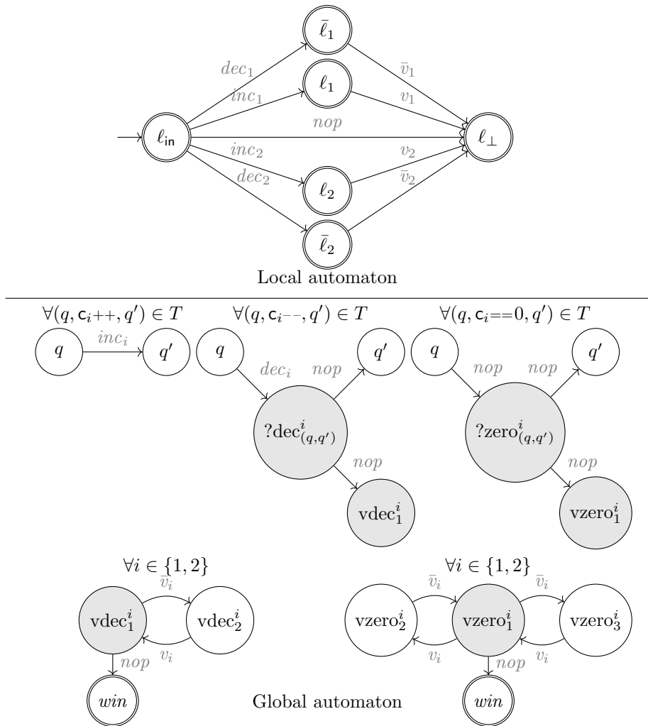
Fig. 6 Construction of \mathcal{G}_{B\text{-cb}}^P . Global states belonging to Player 1 are drawn with a light gray background. Not pictured: q_0 is the initial global state and q_h is accepting.
