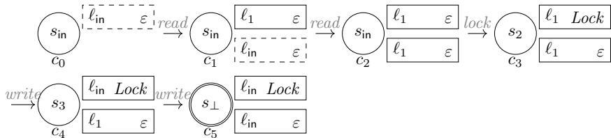
Fig. 2 An example of an accepting finite run involving two processes
