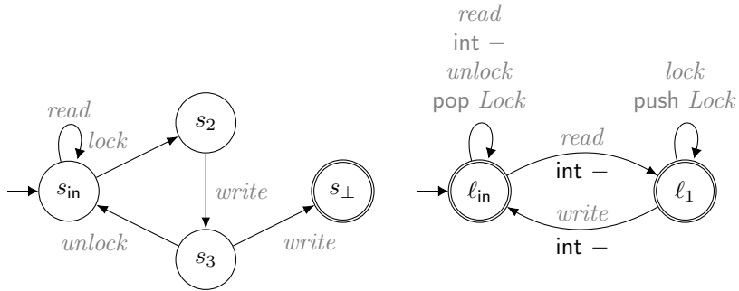
Fig. 1 A DPS represented as a global automaton (left) and local automaton (right) synchronized with labels (in gray)
