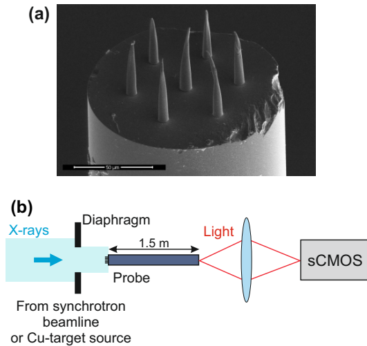
Fig. 1. (a) SEM image of a fiber-integrated multi-pixel detec- tion array on top of a seven-core optical fiber. Each pixel is in direct optical coupling with one of the fiber core. (b) Scheme of the experimental set-up for the detector demonstration.
