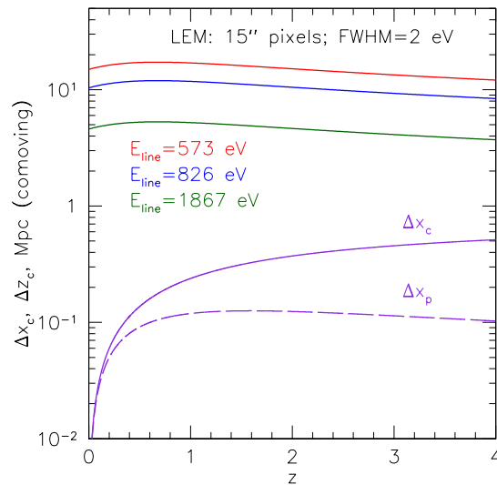
Fig. 17 — LEM "3D" spatial resolution as a function of redshift. The violet lines show the comoving (Δx c , the solid line) and physical sizes (Δx p , the dashed line) corresponding to 15" pixels. The other three lines show the effective resolution along the lines of sight, corresponding to the comoving distance between objects in the Hubble flow.
