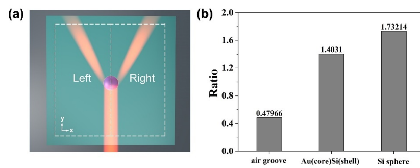
Figure S2 The electric field excited by the nanoparticle and the electric field on the surface of the 1D-PC without nanoparticle under the illumination of circularly polarized Gaussian beam at normal incidence.
