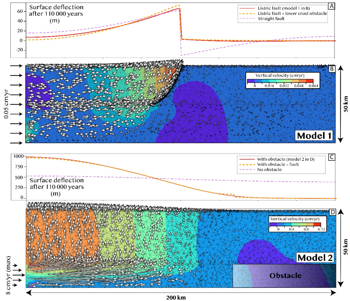
Figure 3. A/ Surface deflection and B/ velocity field of model 1, deforming under constant horizontal velocity boundary condition, and a fault embedded in the upper crust. C/ Surface deflection and D/ Velocity field of model 2, deforming under Poiseuille flow condition in the lower crust.
