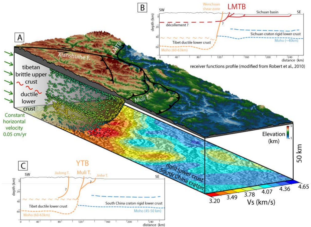
Figure 4. A/ 3D block diagram of the Yalong margin with surface topography (2X vertical exaggeration, Pitard et al., 2021), tomography section at 50 km-depth (Yao et al., 2008), and the 2D crustal velocity field of our model 1, with constant lateral push, where shallow the high angle listric Muli thrust acts as a ramp to exhume crustal material. B/ 2D vertical section across the LongMenShan Thrust Belt (LMTB) drawn from the receiver function profile of Robert et al. (2010). C/ 2D vertical section across the Yalong margin, modified from B, showing a similar crustal geometry inferred for the Yalong Thrust Belt (YTB).
