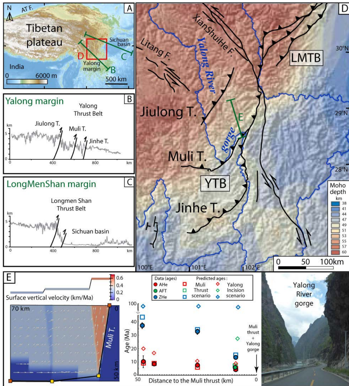
Figure 1. A/ Location of the Yalong margin, South-East Tibet. AT F.: Altyn Tagh fault. B/ & C/ Topographic profiles across the Yalong and the LongMenShan margins (see A/ for location). D/ Moho depth map (Yao et al., 2008), with main faults, LMTB : Longmenshan thrust belt, YTB : Yalong thrust belt including the Jiulong, Muli and Jinhe thrusts (T.), XianShuiHe and Litang strike-slip faults (F.). E/ 2-D crustal velocity field obtained by inversion of thermochronology ages with corresponding measured and predicted ages (AHe and ZHe: Apatite or Zircon (U-Th)/He, AFT: Apatite fission track) for the tectonics
