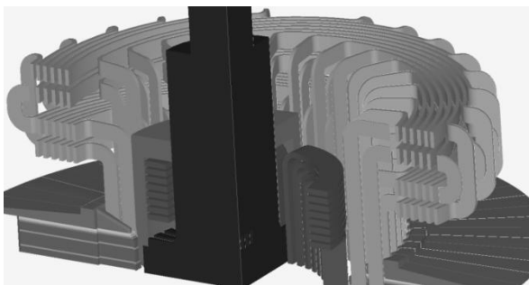
Fig. 1. Finite element model of the 125 MW turbo-generator end-region.
