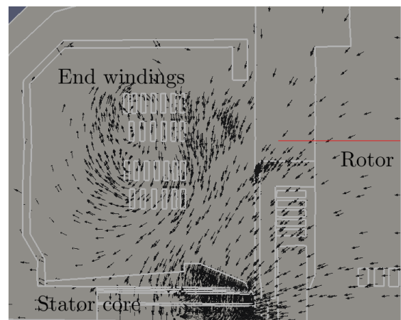
Fig. 2. \mathbf{H} field map in the end-region of the turbo-generator (cf. figure 1).
