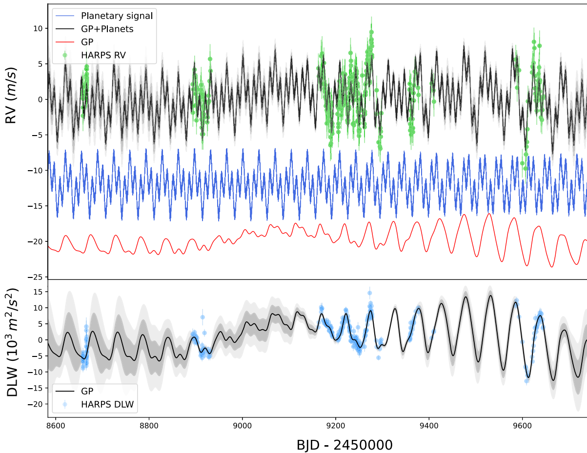
Figure 8. RV and differential line width (DLW) time series with best-fitting models from the multi-GP (solid black lines) and the corresponding GP models (light gray shaded areas). The upper panel shows the RV data with the full model in black, while the planetary signal (blue), and stellar (red) inferred models are shown with a vertical offset for clarity. The lower panel shows the DLW along with the stellar inferred model. Data are shown with filled circles, with their nominal error bars and semitransparent error bar extensions accounting for the inferred jitter term.
