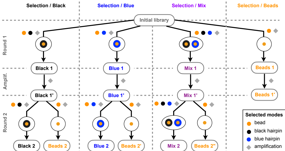
FIG. 6. Training the model: selected set of modes. The selected modes incorporated in the model vary with each specific round. This adaptability enables comprehensive training using all available data. In the figure, the tree structure of the experiment (as presented in Figure 1 of the main text) is reported with the annotations of the selected mode for each branch or selection round. The four modes model distinct physical processes depicted in Fig. 5: binding the black hairpin, binding the blue hairpin, binding the supporting bead, and the bias introduced during the amplification process.
