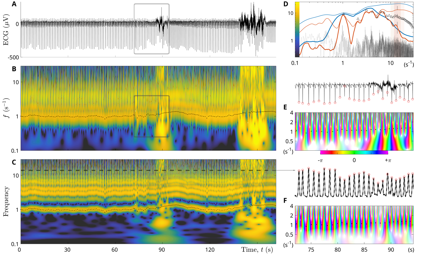
Figure 4: (A) ECG signal x(t) ( \mu\text{V} ). (B) |X(t, f; Q)| with Q = 1 . (C) |X(t, f; Q_{\text{qrs}})| with Q_{\text{qrs}} = 3 . The colour scale ( \mu\text{V} ) is aligned with (D). (D) Amplitude spectra: |\hat{x}(f)|/T over one RR interval (black triangles) or the selected time interval (grey line), median (thick lines), and root-mean-square (thin lines) over time of (B, blue) and (C, red). (E) x(t) and X(t, f; Q) (zoom in the boxes in A, B), with modulus-angle colour coding near the heart rate. (F) Amplitude of the QRS complexes y(t) = |X(t, f_{\text{qrs}}; Q_{\text{qrs}})| at f_{\text{qrs}} = 14 \text{ s}^{-1} (grey dashed line in C, D) and Y(t, f; Q) with Q = 1 . Heart rate (dots in B, C, E, F) estimated from detected QRS complexes (red circles in E, F).
