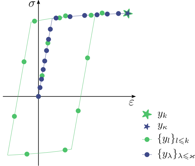
Figure 4: Identical states y_k and y_\kappa in constitutive space (\varepsilon, \sigma) but with different histories.
