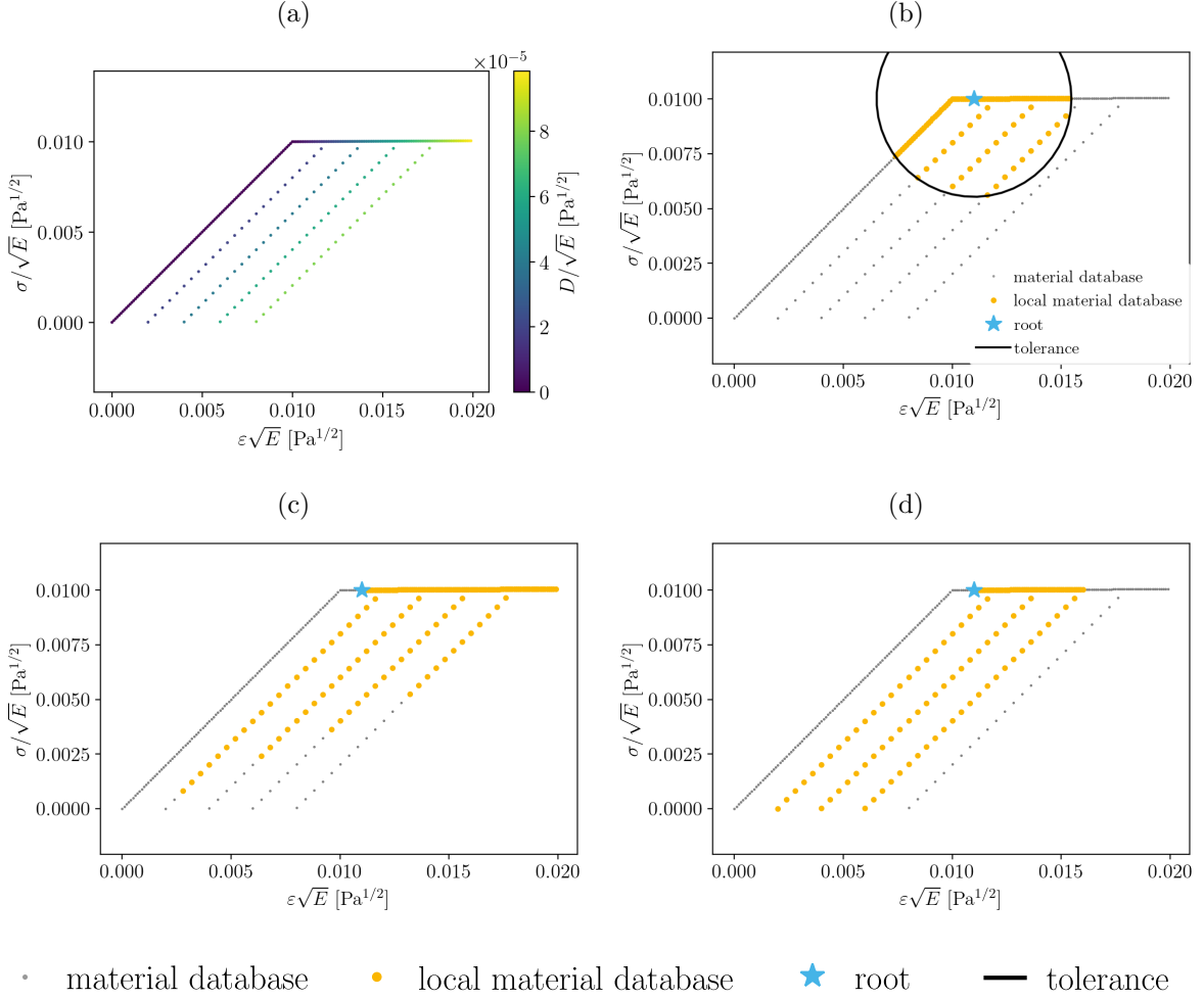
Figure 8: Material database and effect of reduction criteria on the local database. (a) Material database. (b) Data-driven distance, TOL1=10^{-5} \times C . (c) Cumulated data-driven distance along the path, TOL2=10^{-2} \times C . (d) Path dissipative cost, TOL3=5 \cdot 10^{-5} \times C .
