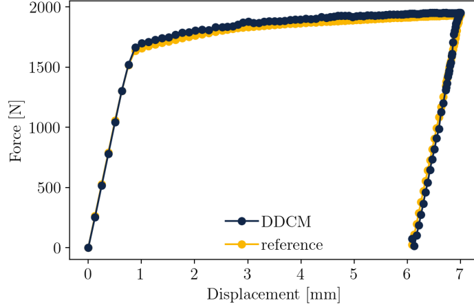
Figure 16: Evolution of resulting force against displacement for the truss problem with predictor-corrector algorithm.
