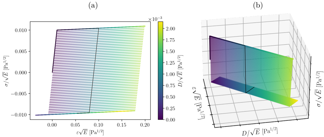
Figure 7: Material data set under loading, unloading and reloading conditions.
