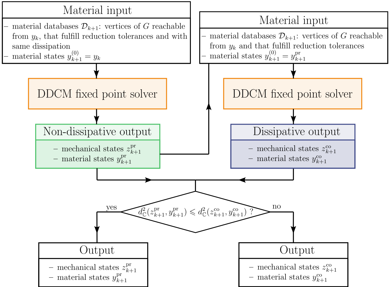
Figure 14: Illustration of the predictor-corrector elastoplastic DDCM algorithm.
