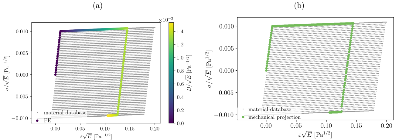
Figure 9: Material data set and (a) FE solution, (b) projected reference mechanical states.
