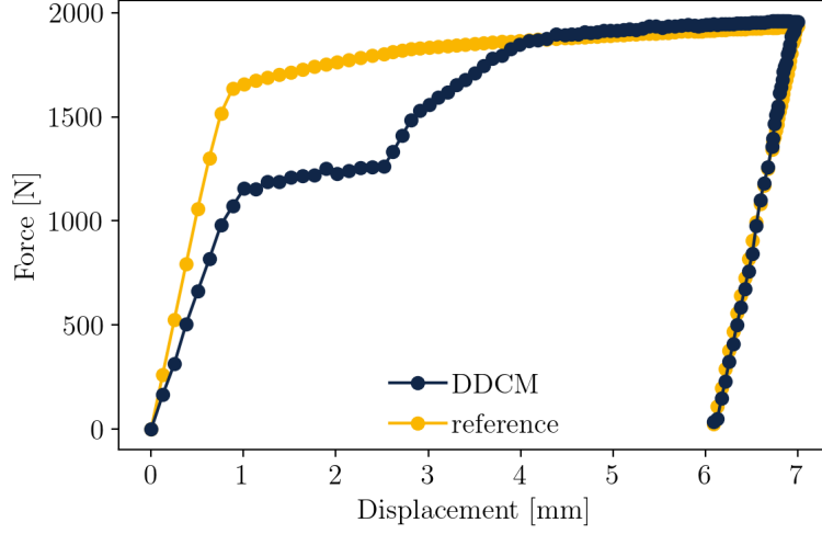
Figure 13: Evolution of resulting force against displacement.
