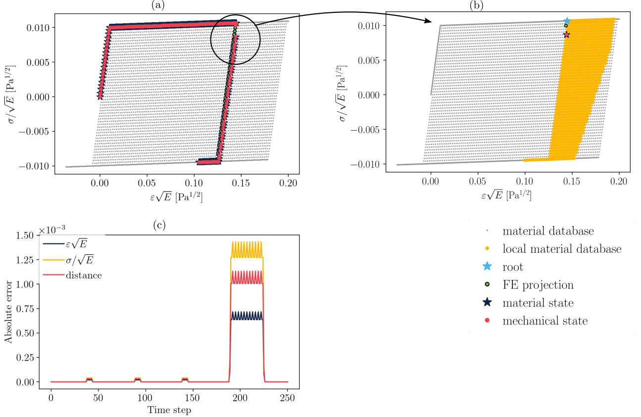
Figure 11: (a) Mechanical and material solutions for the spring-bar element model under loading, unloading and reloading. (b) DDCM solution and projected reference mechanical state at maximum loading. (c) Error between DDCM and projected reference mechanical states.
