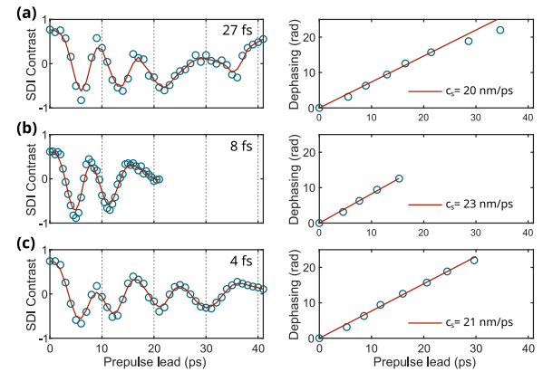
FIG. 3. Experimental SDI contrast curves (left, circles are raw data, lines are smoothed data) and extracted dephasing curves \Delta\phi(\tau) (right, circles are extracted data, lines are linear fits including points with \tau < 20 ps) for SDI scans obtained for driving laser pulse durations of 27 fs (a), 8 fs (b) and 4 fs (c).
