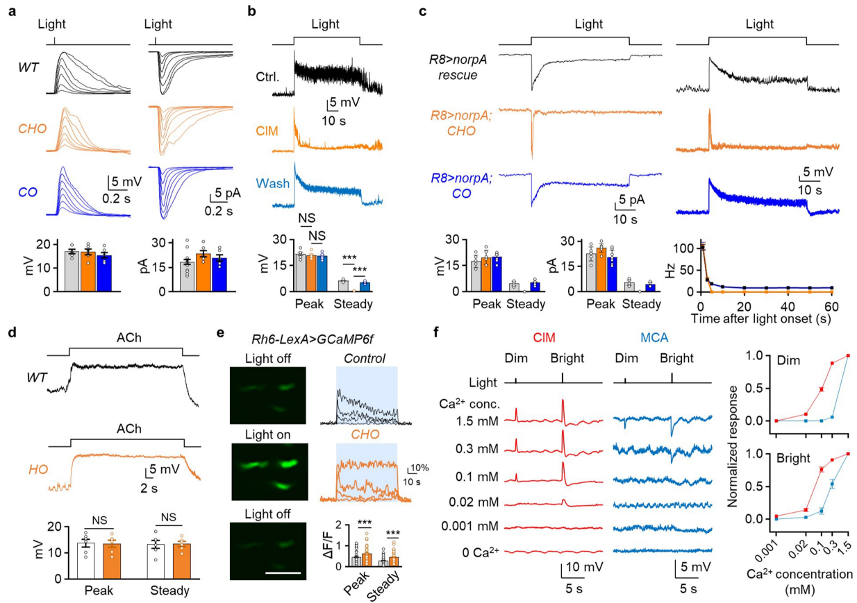
Extended Data Fig. 9 | ACh release sustained by histamine feedback in R8s.
