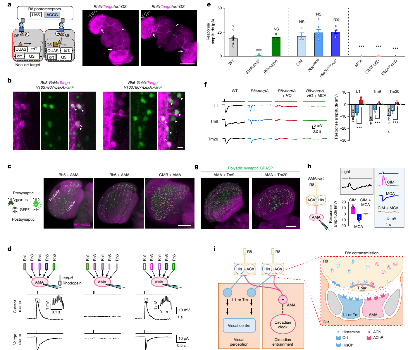
Fig. 3 | ACh and histamine act on distinct neurons. a , ort -independent postsynaptic neurons. Left: schematic of trans -Tango tracing with ort -QS excluding QF-driven tdTomato (tdT.) expression in ort -expressing neurons; right: ort -independent postsynaptic neurons of pR8 and yR8 photoreceptors. Open arrowheads mark multicolumnar arborization, arrows mark accessory medulla innervation, and filled arrowheads mark the arcuate commissure. Scale bar, 100 \mu m. b , VT037867-labelled neurons overlap with ort -independent postsynaptic neurons of pR8 (left) and yR8 (right) photoreceptors. Arrowheads mark co-labelled cells. Scale bar, 5 \mu m. c , Connections between R8 photoreceptors and AMA neurons. Left: schematic of GRASP labelling; right: GRASP between AMA neurons and pR8 ( Rh5-Gal4 ), yR8 ( Rh6-Gal4 ) or all ( GMR-Gal4 ) photoreceptors. Scale bar, 50 \mu m. d , AMA neurons are excited by R8 photoreceptors. Top: schematic of photoreceptor manipulation: wild-type flies (left), Rh5 2 ;Rh6 1 flies (middle) and norpA PA1 flies with norpA rescued in R8 photoreceptors (right). Middle: representative light-induced depolarization; insets represent spikes outlined by the dashed line. Bottom: representative
