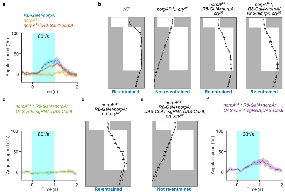
Extended Data Fig. 3 | R8s use histamine for motion detection and ACh for circadian photoentrainment. a , Motion detection by R8s to slow ( 60^\circ/\text{s} ) visual stimuli. Pooled angular speed in norpA P41 ( n = 10 ), R8-Gal4 ( Rh5-Gal4 , Rh6-Gal4 )> norpA ( n = 12 ), and norpA P41 ; R8-Gal4 > norpA ( n = 11 ) flies. Data are represented as mean (solid line) and s.e.m. (shading). b , Circadian photoentrainment by R8s. Phase plots of evening peaks of wild-type flies (left, n = 33 ), norpA P41 ; cry 02 mutant flies (second panel from left, n = 102 ), the flies with only R8s and H-B eyelets in dim-light detection (third panel from left, n = 93 ), and the flies with only R8s in dim-light detection (with H-B eyelets
