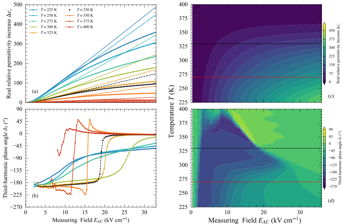
Figure 3. Relative permittivity variation (a)-(c) and phase angle of the third harmonic (b)-(d) as a function of the AC measuring field for different values of the temperature. For relative permittivity presented in (a), dots correspond to the experimental data and the solid lines to the hyperbolic fits. The black dashed line corresponds to T_{max} (at E_{AC} = 0.3 \text{ kV cm}^{-1} ). The red dashed line in (c)-(d) corresponds to the inflection point at T = 270 \text{ K} . Data presented in (a)-(b) corresponds to slices every 25 K of the data presented in (c)-(d).
