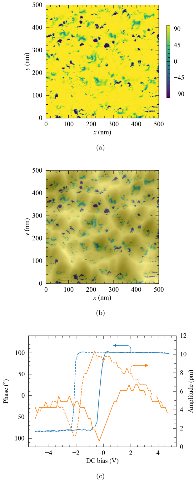
Figure 1. Phase of the Vertical PFM (VPFM) (a). Superimposition of the phase signal and the topography (b). PFM phase and amplitude as a function of an applied DC voltage V_{DC} (c).
