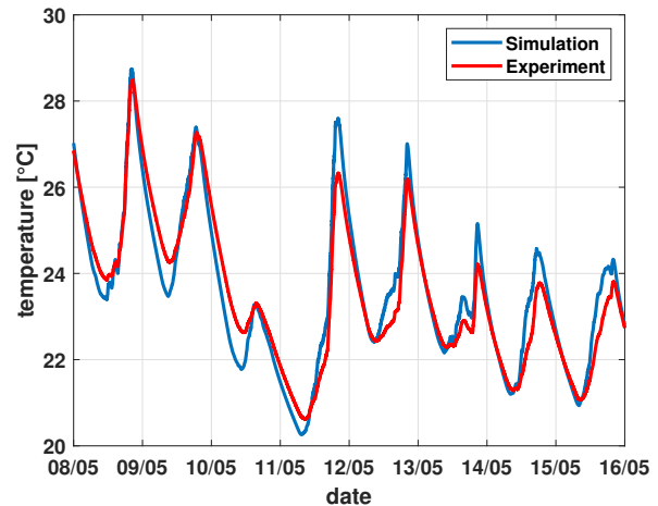
Figure 8: Measured and simulated surface temperature at probe 7 (on the North wall).
