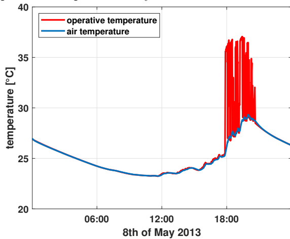
Figure 11: Air temperature and operative temperature in the middle of the room.
