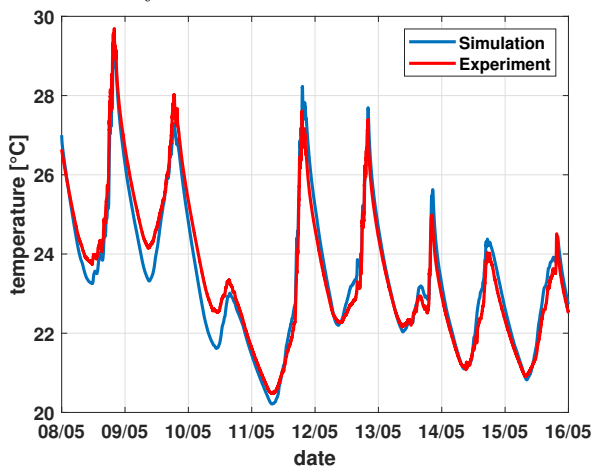
Figure 10: Measured and simulated room air temperature.
