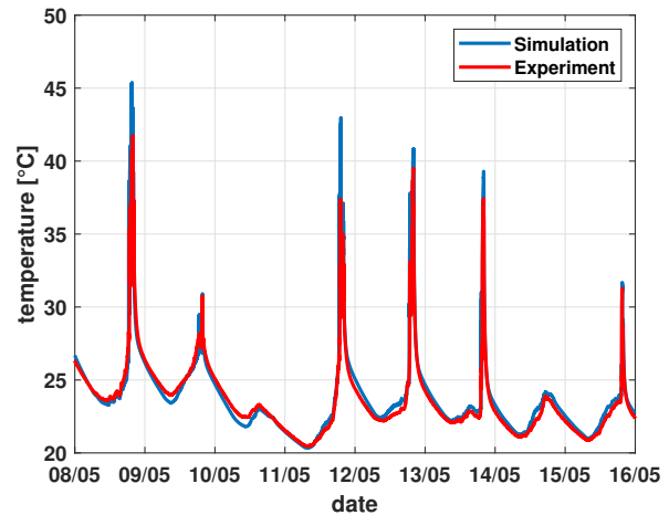
Figure 6: Measured and simulated surface temperature at probe 2 (on the East wall).
