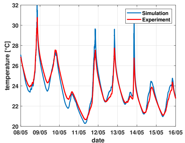
Figure 7: Measured and simulated surface temperature at probe 4 (on the South wall).
