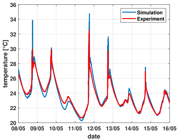
Figure 9: Measured and simulated surface temperature at probe 8 (on the floor).
