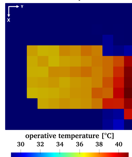
Figure 13: Operative temperature field in the room over the plane P1 the 8th of May 2013 at 5:24 PM.
