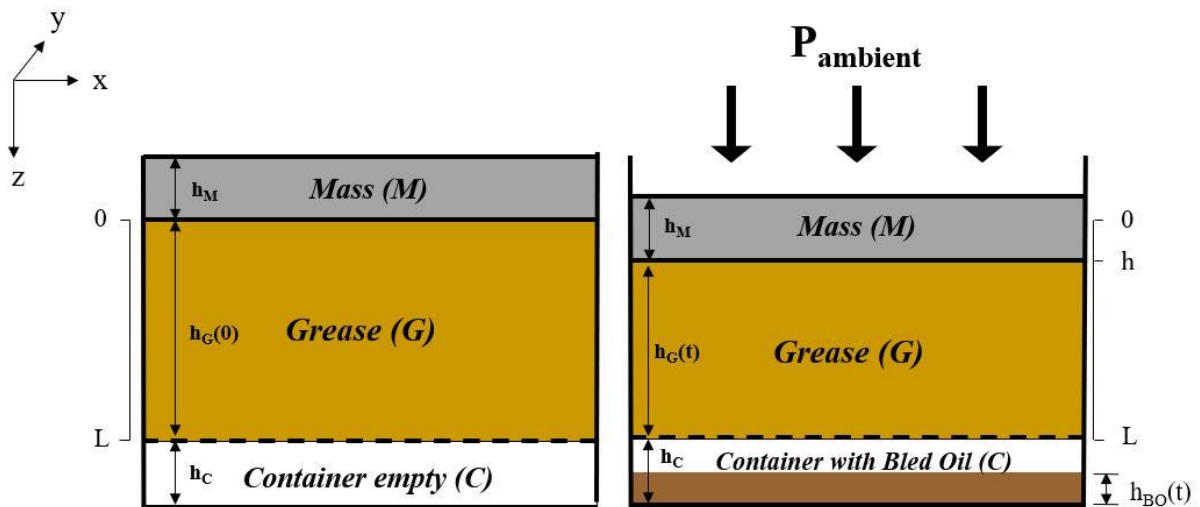
Figure 3: One-dimensional (1D) schematic view of the system evolution under gravity and pressure forces with on the left side, the initial state ( t=0 s) of the system and on the right side, state of the system at time t .
