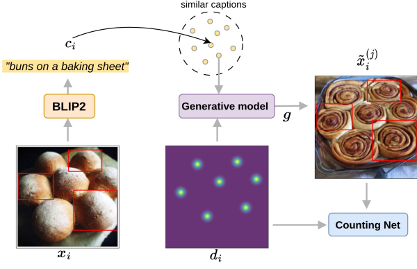
Figure 3. Overview of our approach. We condition a pre-trained diffusion model on both text prompts and density maps and perform swaps with similar captions. The density and original exemplar boxes are used as ground-truth for the generated augmentation.
