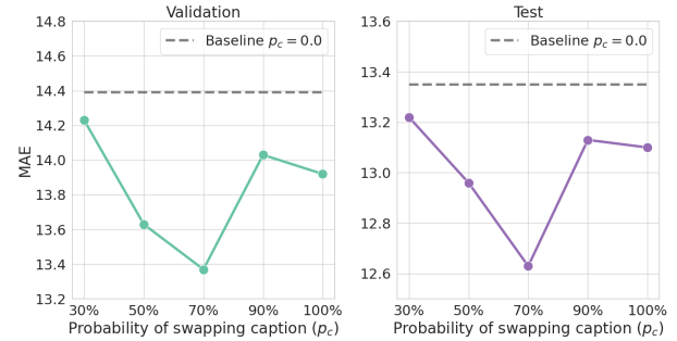
Figure 8. Impact of the percentage of diverse augmentations p_c on SAFECOUNT. MAE is reported for the val and test sets of FSC147.
