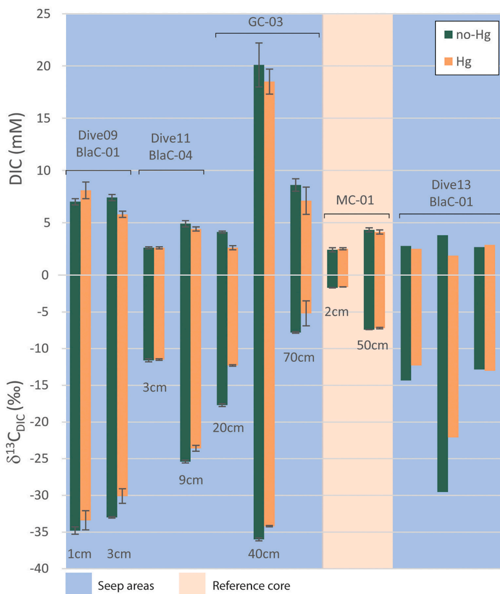
Fig. 3. Comparison of the DIC concentration and carbon isotopic composition ( \delta^{13}\text{C}_{\text{DIC}} ) of pore water samples with \text{HgCl}_2 addition ( Hg ) and without it ( no-Hg ). Error bars correspond to the 1 standard deviation of replicates.
