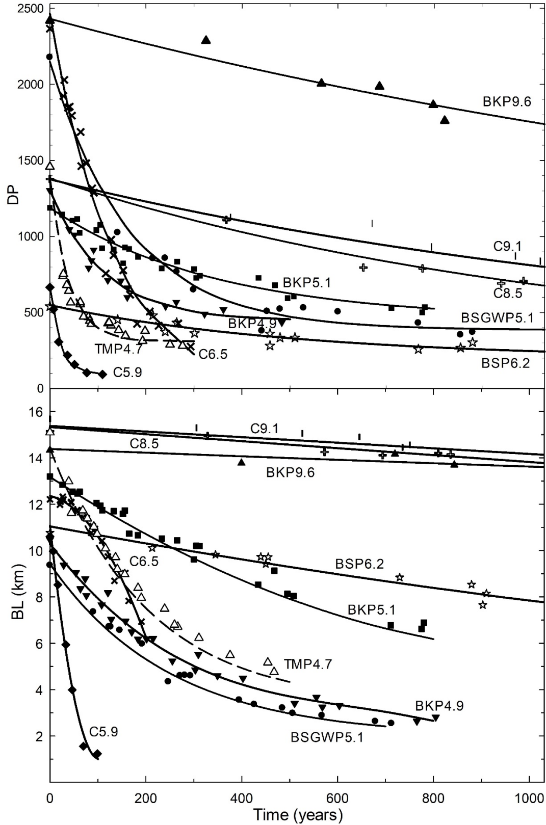
Fig. 1 DP and BL decay over time obtained by the extrapolation of artificial ageing conditions to 21 °C and 50% RH
