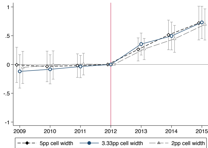
(a) Varying cell width for (2.2,2.8) window
