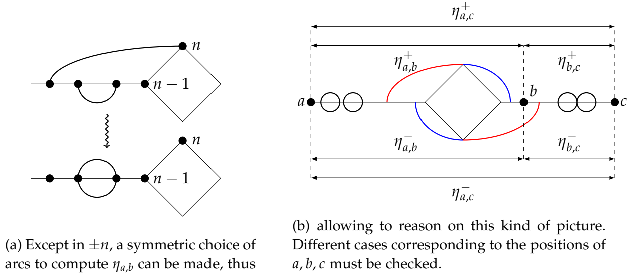
Figure 3: Idea of proof for Lemma 13.
