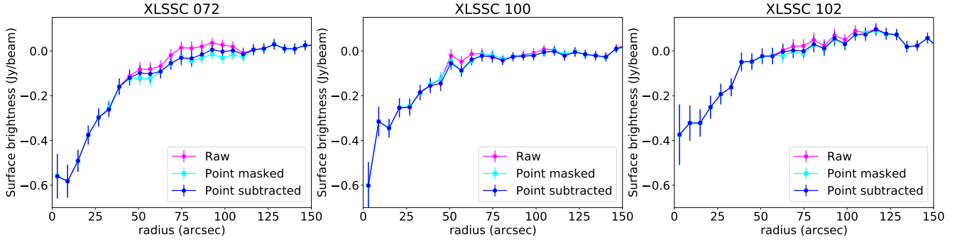
Fig. B.3. Comparison of 150 GHz surface brightness profiles when accounting (or not) for the point sources.
