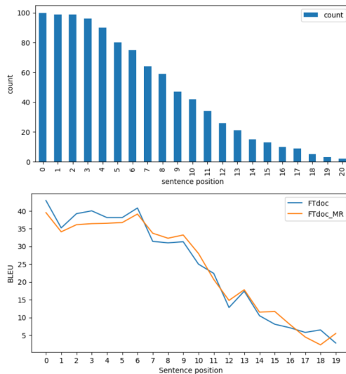
Figure 5. Evaluation of sentences in THE_{doc} with respect to their position in the document.
