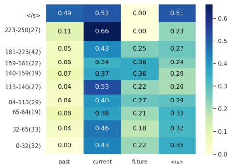
Figure 3. An example of attention distribution on past, current and future source sentences in a document with 9 sentences. The last column indicates the target attention on source EOS tag.
