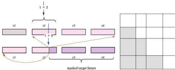
Figure 1. Decoder-side attention represented by brown arrows (left) and the context mask (right) for FTdoc_maskPast
