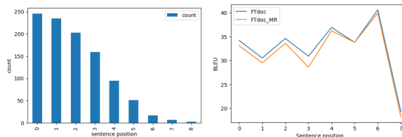
Figure 6. Evaluation of sentences in TAL_doc with respect to their position in the document.
