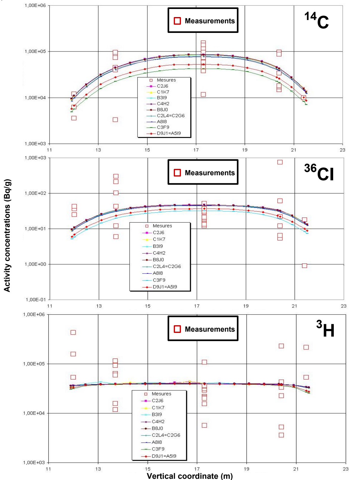
Figure 3: Activity concentration profiles calculated by the proposed method. y axis are Bq/g of ^{14}\text{C} , ^{36}\text{Cl} and ^3\text{H} versus x axis which is vertical coordinate of the Bugey 1 graphite pile with squares representing sample measurements, compared to average calculated curves for the 11 corresponding sampled channels. The more or less parabolic shapes of the calculated profiles are fully explained by the neutron capture cross section of the explanatory impurities ( ^{13}\text{C} , ^{35}\text{Cl} and ^6\text{Li} )
