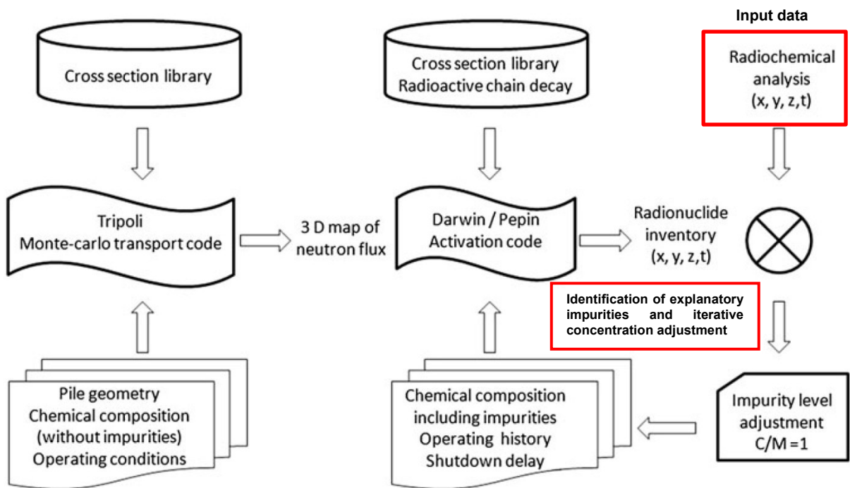
Figure 2: Simplified description of step 1 and step 2 principles for calculating the radionuclide inventory of the piles in the EDF reactors by identification method
