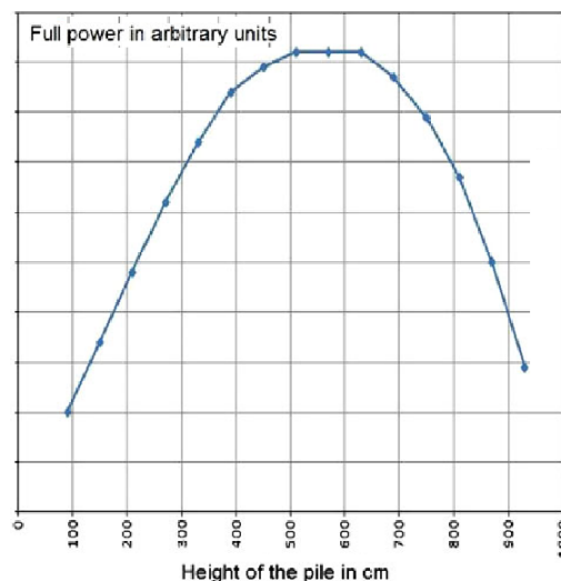
Figure 1: Shape of the thermal power correlated to the neutron flux into a fuel channel of the Bugey 1 reactor with x axis height of the pile in cm and y axis full power in arbitrary units
