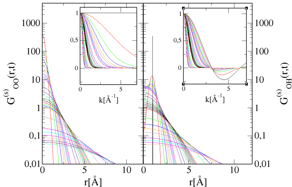
Figure 13: Ethanol: comparison of Self correlations G^{(s)}(r, t) and F^{(s)}(k, t) (inset) for oxygen-oxygen (left panel) and oxygen-hydrogen (right panel) pairs of sites. The lines correspond to the 29 times selected (see text for curve plotting conventions). Note the vertical log-scale for the main panel.
