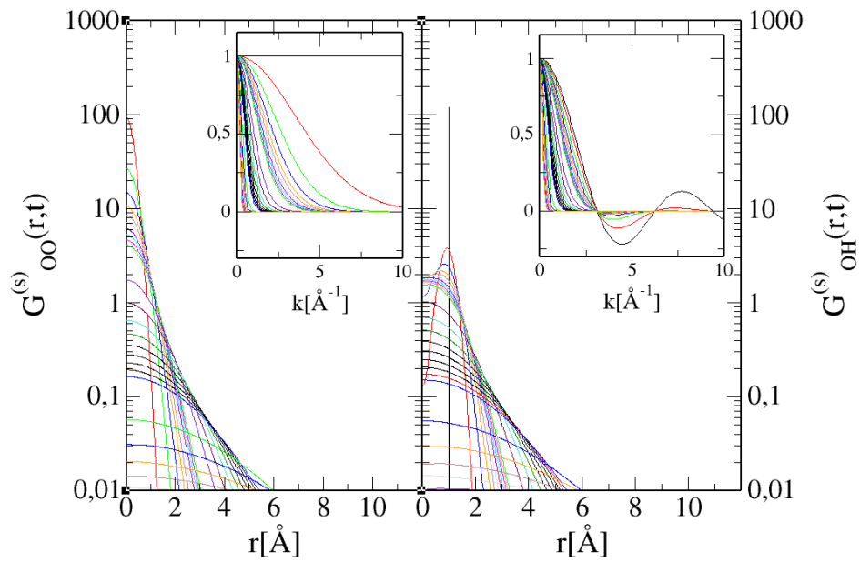
Figure 9: Water: comparison of Self correlations G^{(s)}(r, t) and F^{(s)}(k, t) (inset) for oxygen-oxygen (left panel) and oxygen-hydrogen (right panel) pairs of sites. The lines correspond to the 29 times selected (see text for curve plotting conventions). Note the vertical log-scale for the main panel.
