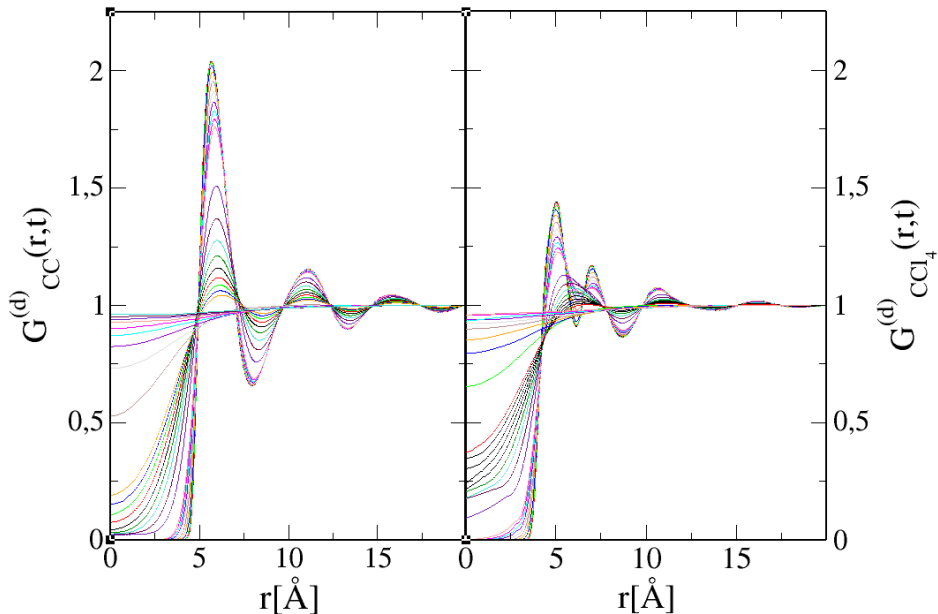
Figure 2: \text{CCl}_4 : comparison of distinct van Hove functions G^{(d)}(r, t) for carbon-carbon (left panel) and carbon-chloride (right panel) pairs of sites.
