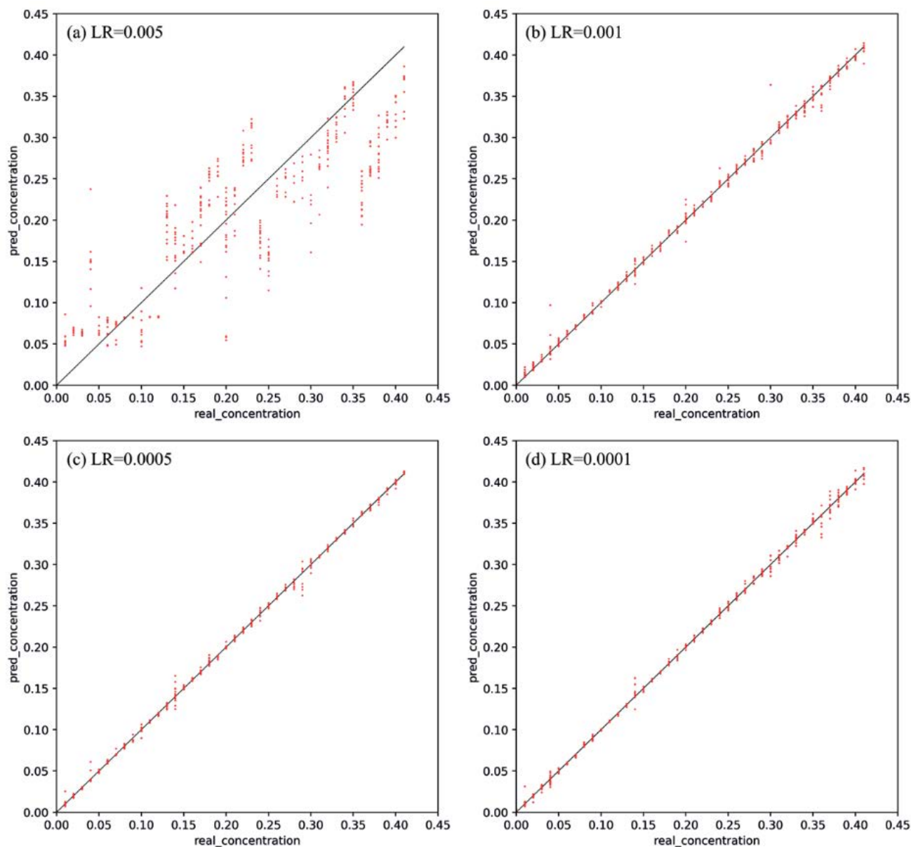
Fig. 7. Comparison of the prediction results by MLF-1DCNN model with different learning rates.
