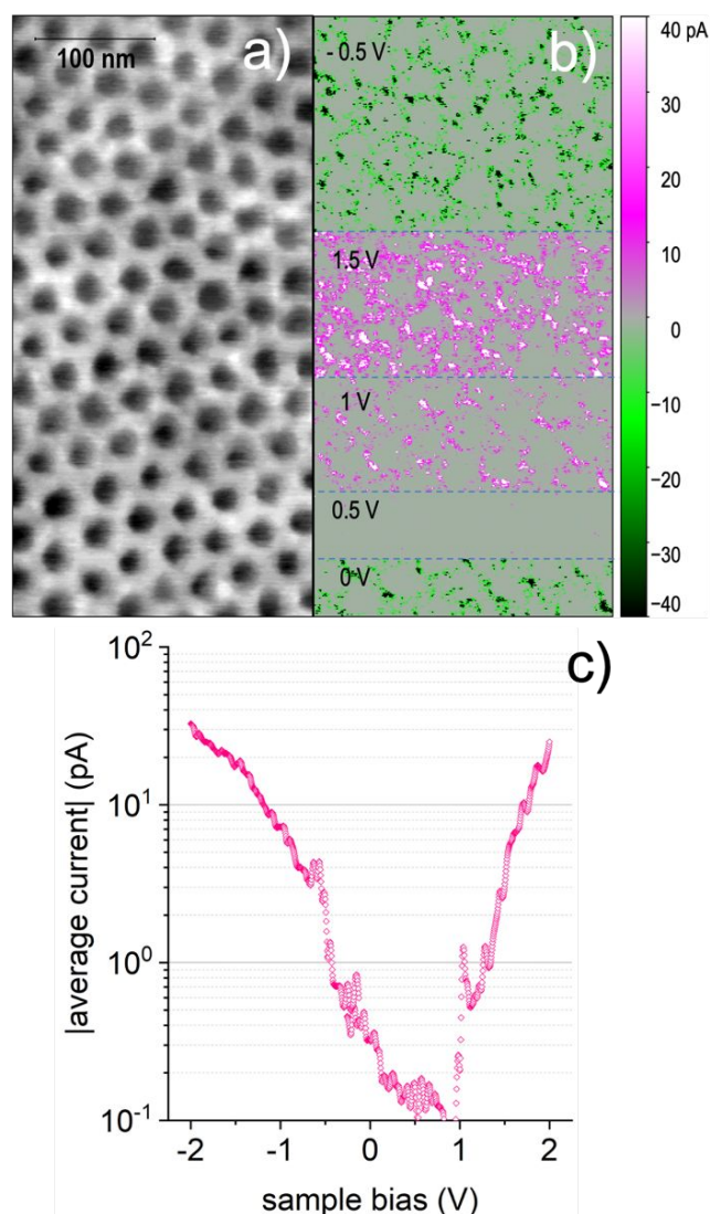
19 20 21 22 23 24 25 26 27 28 29 30 31 32 33 34 35 36 37 38 39 40 41 42 43 44 45 46 47 48 49 50 51 52 53 54 55 Figure 10 Surface morphology (a) and corresponding current map (b) measured on sample with 3.20 \times 10^{14} 56 cm -2 dose, while changing the sample voltage bias as reported in the image. The greyscale of the 57 morphology image corresponds to 3 nm. C) absolute average current vs sample bias voltage in semi-log 58 scale; the current data are obtained averaging over 60 I-V measurements taken at different surface sites. 59 60
