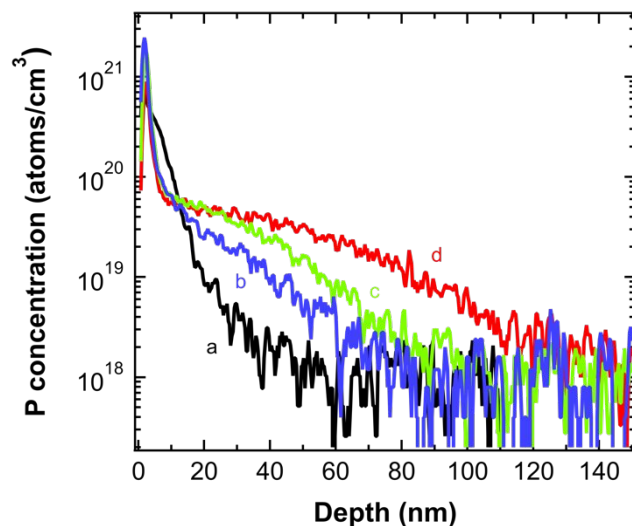
Figure S5. Calibrated profile of P for the sample implanted with dose 1.55 \times 10^{14} \text{ cm}^{-2} . Curves represent the sample (a) before the annealing, after 5 s annealing at (b) 1000 °C, (c) 1050 °C, (d) 1100 °C.
