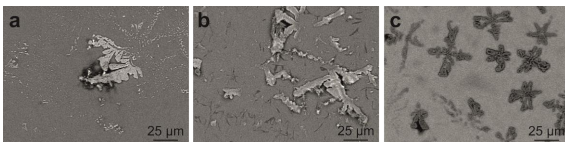
Fig. 3. SEM images of glass samples after 36 days at 100 % RH: a) NCS1, b) KCS1, c) PS1.
