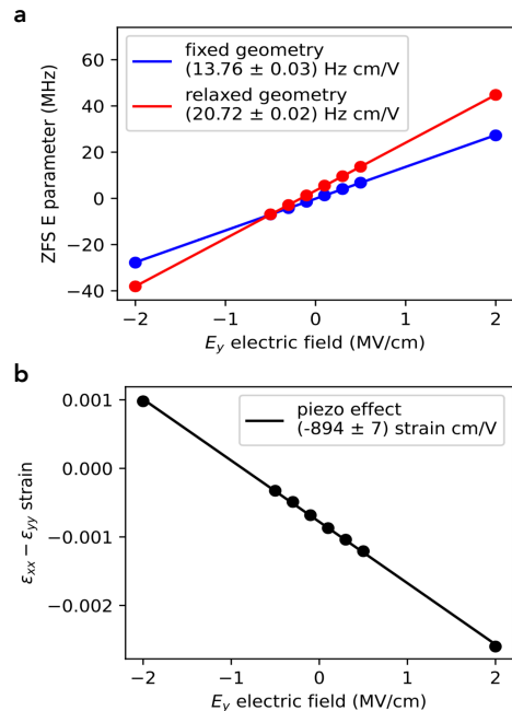
FIG. 3. Response to an external electric field component \mathcal{E}_y . a Orthorhombic ZFS parameter E as a function of the external electric field. The cases of fixed and relaxed atomic positions are compared (blue and red points). b Estimated local strain from the piezo effect induced by the external electric field.
