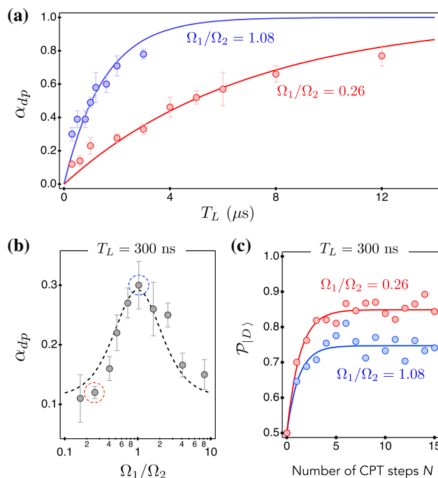
Fig. 7 a Probability \alpha_{dp} as a function of the duration T_L of the laser pulse obtained for \Omega_1/\Omega_2 = 0.26 (red) and \Omega_1/\Omega_2 = 1.08 (blue). Solid lines are data fitting with Eq. (17). b Probability \alpha_{dp} plotted as a function of \Omega_1/\Omega_2 on a semi-log scale for a laser pulse duration fixed to T_L = 300 ns. The black dashed line is a fit to the data using Eq. (20). c Probability \mathcal{P}_{|D\rangle} to find the ^{13}\text{C} nuclear spin in the dark state after N pumping steps for a dual microwave \pi -pulse characterized by \Omega_1/\Omega_2 = 0.26 (red) and \Omega_1/\Omega_2 = 1.08 (blue) using T_L = 300 ns. Solid lines are data fitting with Eq. (19)
