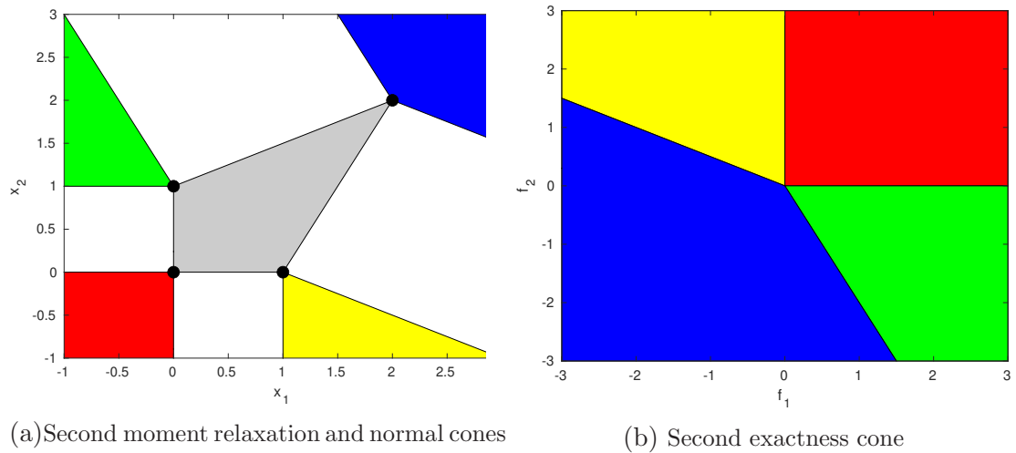
Figure 2: Finite set. Left (a): second moment relaxation (light gray) which is the convex hull of \mathcal{X} (four black points), and normal cones at the points (colored). Right (b): second exactness cone (colored).
