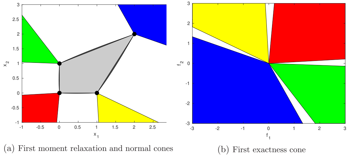
Figure 1: Finite set. Left (a): first moment relaxation (dark gray) including the convex hull (light gray) of \mathcal{X} (four black points), and normal cones at the points (colored). Right (b): first exactness cone (colored).
