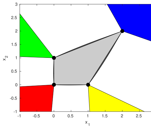
(a) First moment relaxation and normal cones
