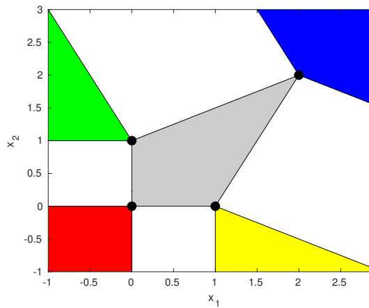
(a) Second moment relaxation and normal cones
