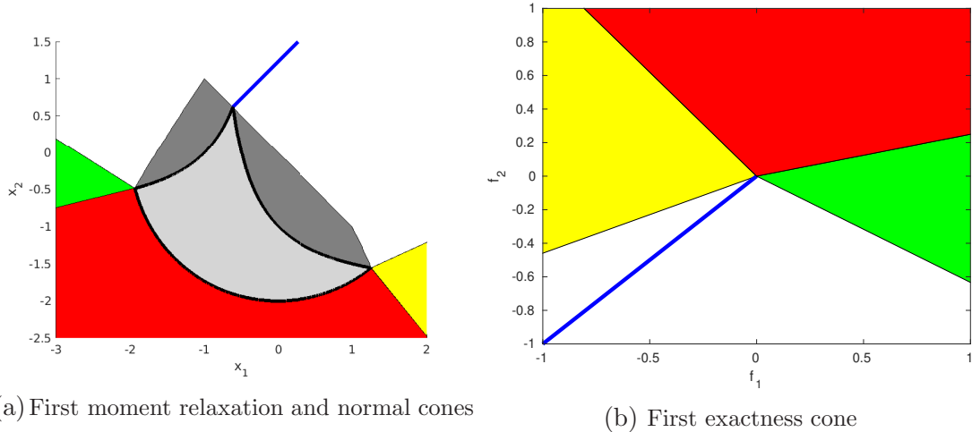
Figure 3: Non-convex set. Left (a): first moment relaxation (dark gray) of \mathcal{X} (light gray), and normal cones (colored). Right (b): first exactness cone (colored).
