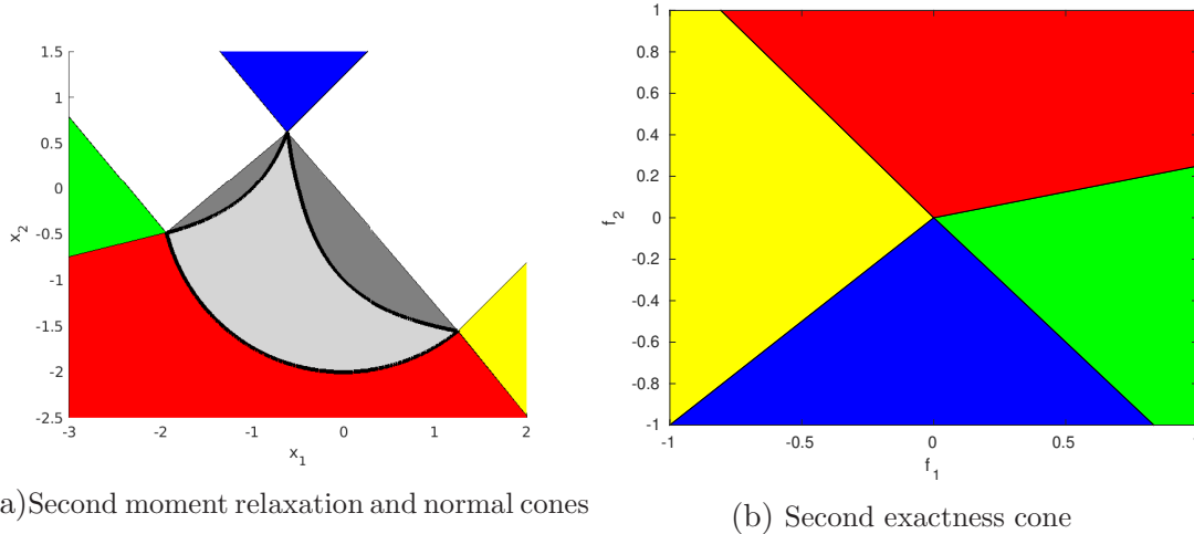
Figure 4: Non-convex set. Left (a): second moment relaxation (dark gray) which is the convex hull of \mathcal{X} (light gray), and normal cones at the points (colored). Right (b): second exactness cone (colored).
