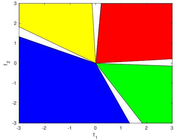
(b) First exactness cone
