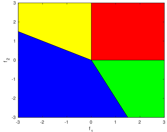
(b) Second exactness cone
