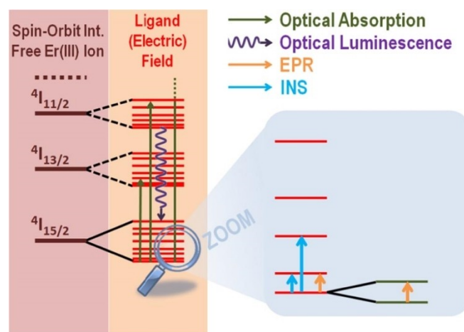
Figure 12. Energy level scheme of \text{Er}^{\text{III}} ion with the energy levels involved in optical, neutron and magnetic resonance spectroscopic techniques. Reproduced with permission from [52c] copyright 2015 IOP.
