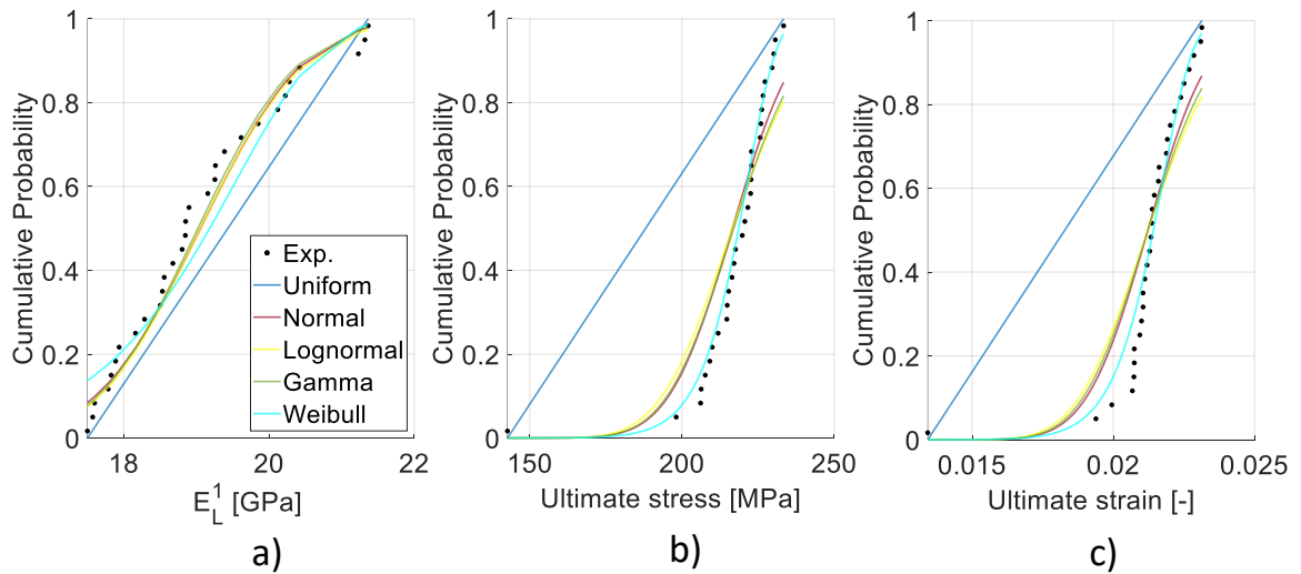
Figure 4. Plot of the experimental dataset and of the cumulative probability functions fitted using usual distribution laws in the case of modulus E_L^1 a), ultimate stress b) and ultimate strain c) for hemp fibre composite.
