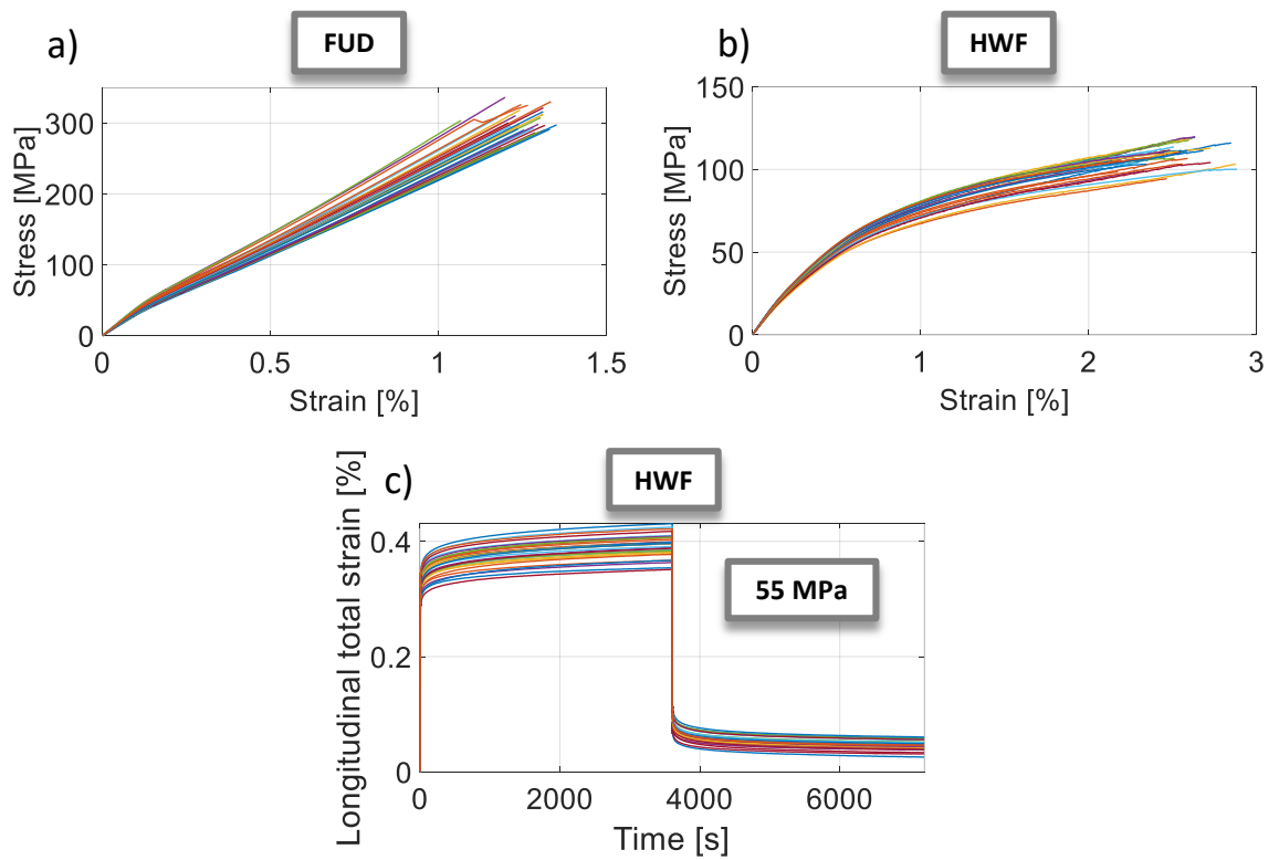
Figure 2: Quasi-static tensile test curves recorded on two batches of 30 FUD a) and HWF b) composite specimens and creep/recovery curves recorded on a batch of 30 samples of HWF composites loaded at 55 MPa.
