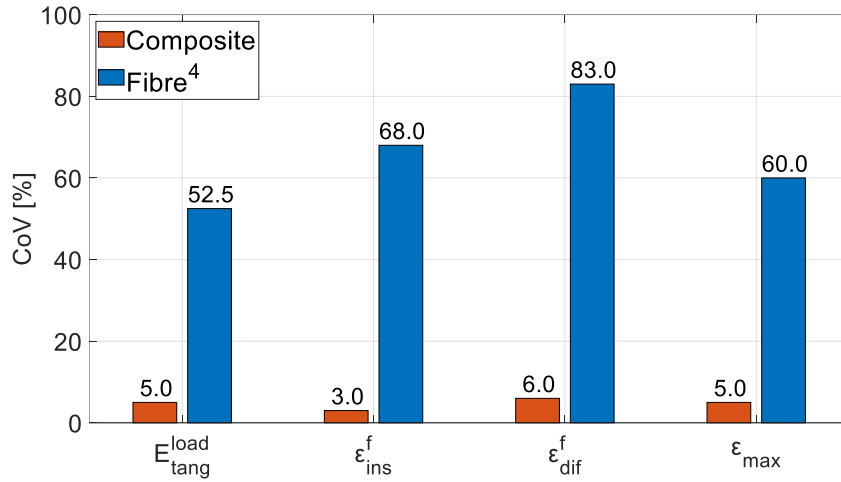
Figure 5. Comparison of the CoV of creep parameters with values from literature at hemp fibre scale ( 4 Cisse et al. [17])
