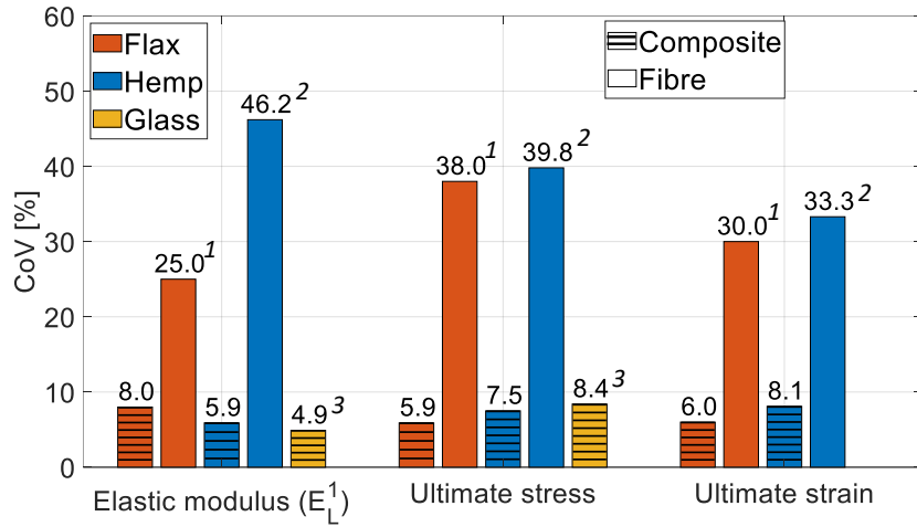
Figure 3: Coefficient of variation of the elastic properties measured on 30 different FUD and HWF composite specimens. Comparison of the value obtained to the ones published in literature for flax fibres ( 1 Lefevre et al. [5]) and hemp fibre (Placet et al.[21]) and glass/epoxy composites ( 3 Blanchard & Sobey [9]).
