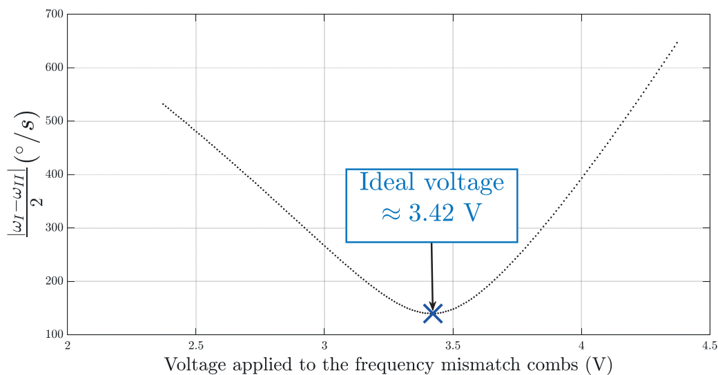
Figure 10. Frequency mismatch minimization experiment on gyroscope n°1.
