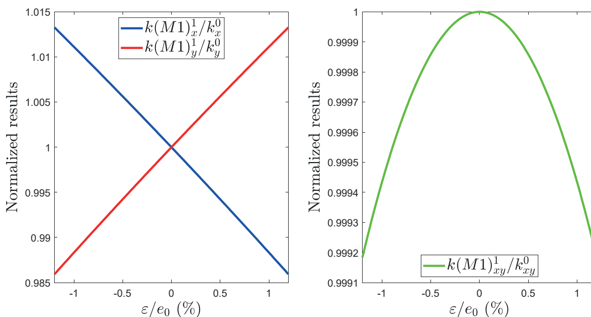
Figure 5. Normalized k(M1)_x^1 , k(M1)_y^1 and k(M1)_{xy}^1 values as a function of the width variation.
