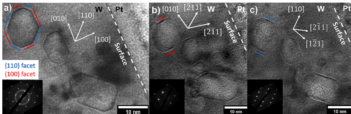
Fig. 2. Bright-field TEM Images of He implanted W(100) annealed up to 1773 K. The three images are taken in the same area from close to the [001] zone axis (a), close to the [102] zone axis (b) and close to the [\bar{1}13] zone axis (c). Faceted He-bubbles are composed of \{110\} and \{100\} facets (in blue and red respectively). Diffraction patterns are shown in the insets, rings are due to polycrystalline platinum (Pt) deposited on the W surface. (For interpretation of the references to colour in this figure legend, the reader is referred to the web version of this article.)
