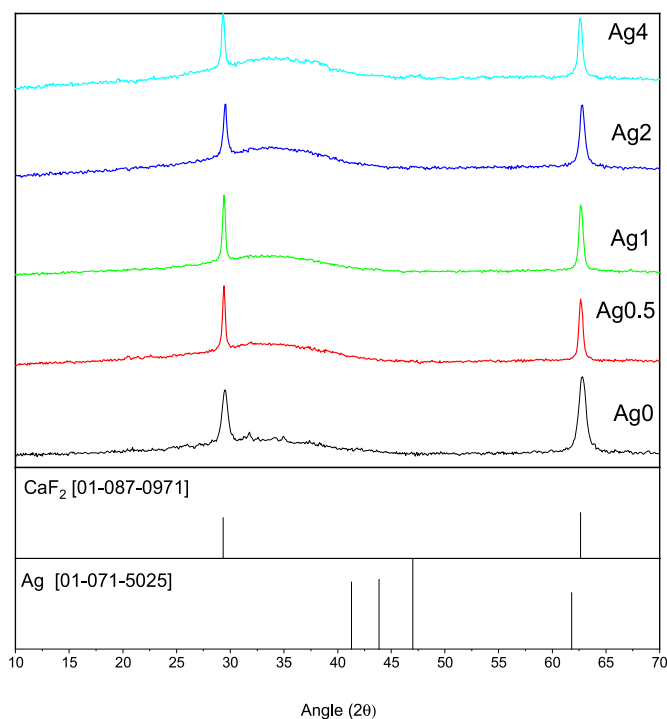
Fig. 5. XRD pattern of the glasses after thermal treatment at ( T_g+20 °C) for 17h and 340 °C for 1h
