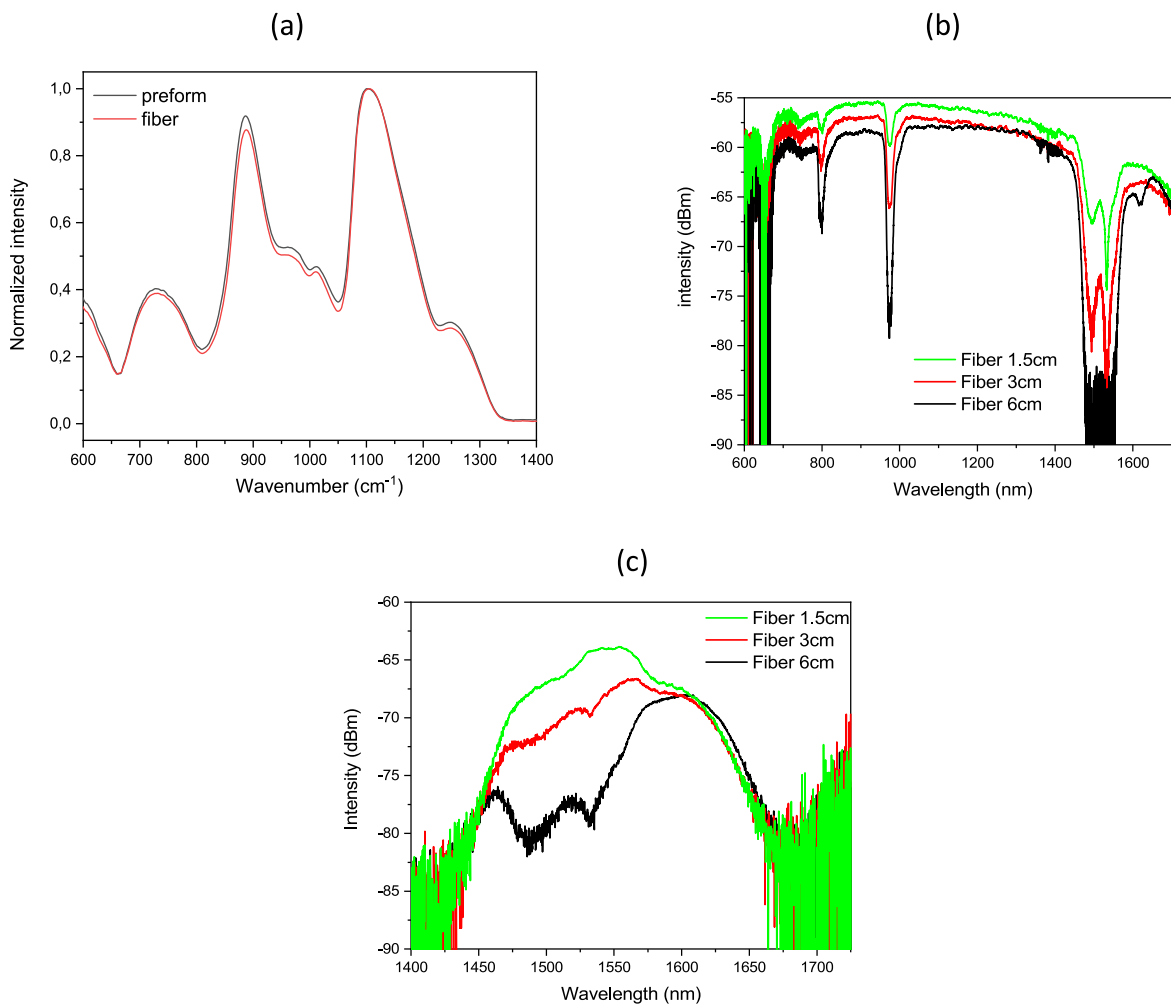
Fig. 10. FTIR (a), Transmittance (b) and Emission (c) spectra ( \lambda_{\text{exc}} = 980 \text{ nm} ) of the as-drawn fibers with different lengths. FTIR spectrum of the preform is also shown in (a).
