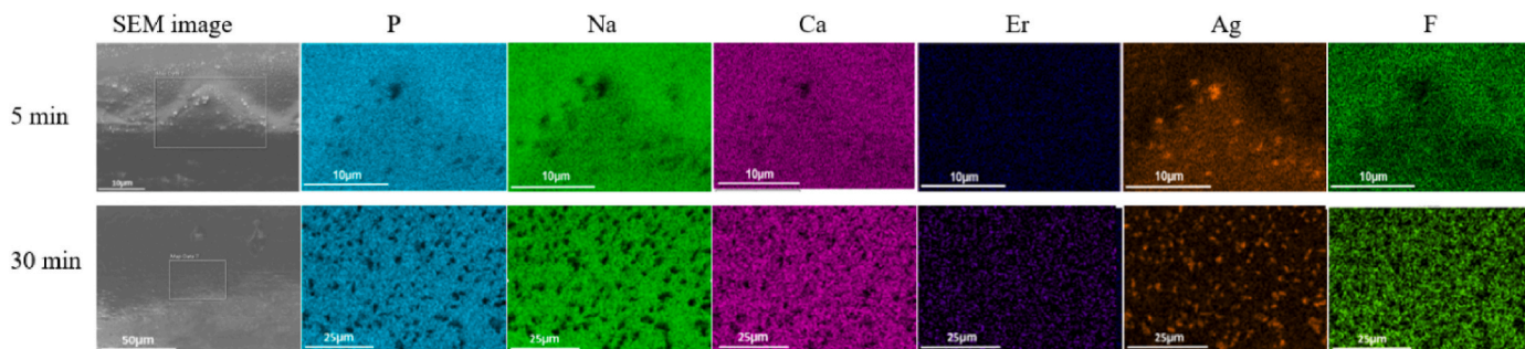
Fig. 13. SEM image of the surface of the fiber heat treated for 5 and 30 min at 300 °C and mapping of the elements.
