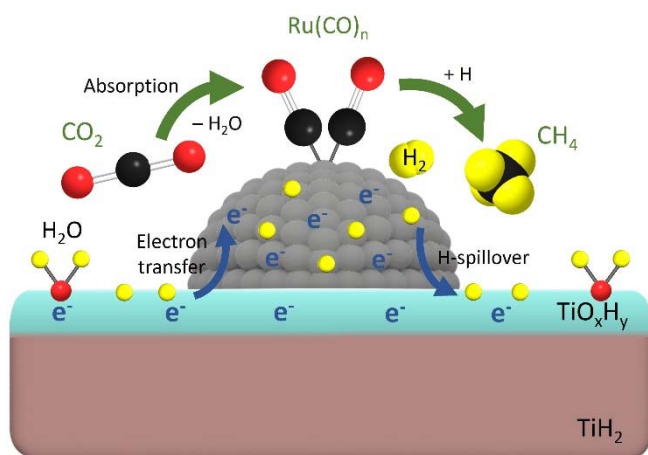
Scheme 1. Proposed relationship between structure, MSI and catalytic performances of m RTH towards \text{CO}_2 methanation.
