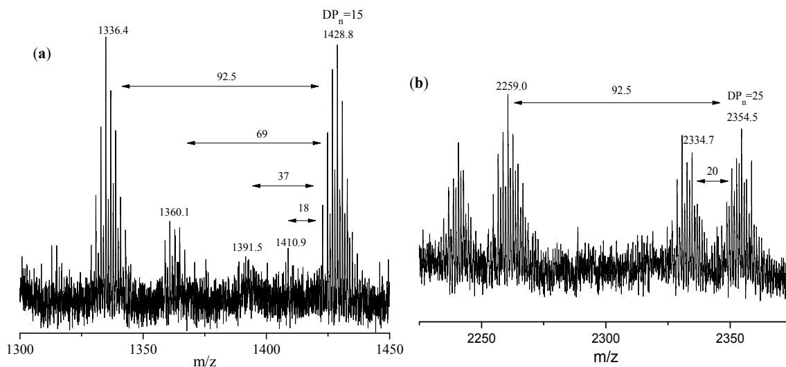
Figure 1. Zooms of (a) low molar mass and (b) high molar mass parts of MALDI TOF MS spectrum of PECH synthesized with BD/BF 3 OEt 2 initiating system (run S17, Table S4). Full spectrum is given in Figure S6.
