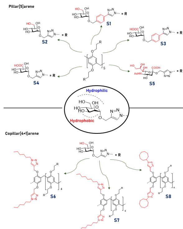
Figure 1. Chemical structures of saccharide homopillar[5]arenes (top) and copillar[4+1]arenes (bottom) and their structural variations (red). The D-mannoside configured carbohydrates display a hydrophobic membrane binding \alpha -face and a hydrophilic water binding \beta -face.
