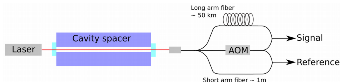
Figure 1: A laser is stabilized on an ultra-stable cavity, and the transmitted light is injected into a three-arm fibered interferometer. The reference is given by the interferometric signal from the AOM – "short" arm comparison, while the signal possibly perturbed by dark matter will be given by the AOM- "long" arm interferometric signal.
