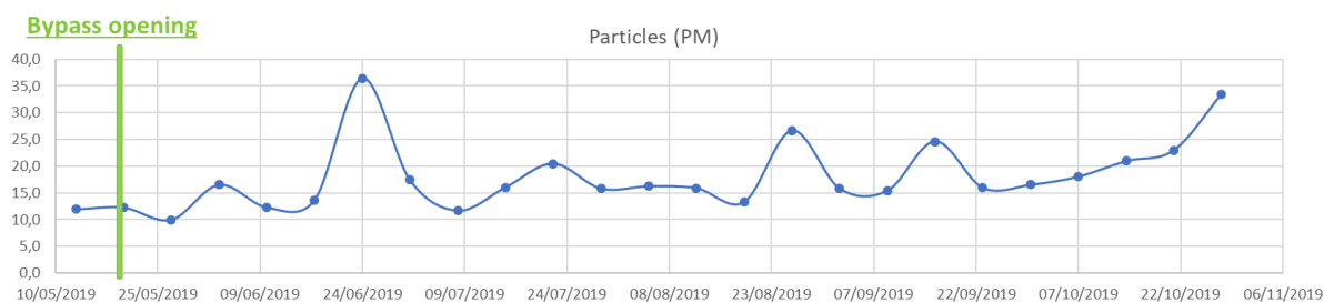
Figure 13 (a): PM level measured by the town center air monitoring micro - station before and after the bypass opening (based on weekly averages).
