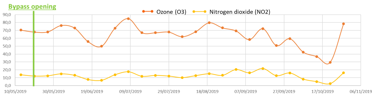
Figure 13 (b): O 3 and NO 2 levels measured by the town center air monitoring micro - station before and after the bypass opening (based on weekly averages).
